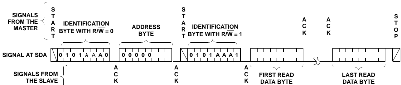
FIGURE 18. RANDOM ADDRESS READ SEQUENCE
