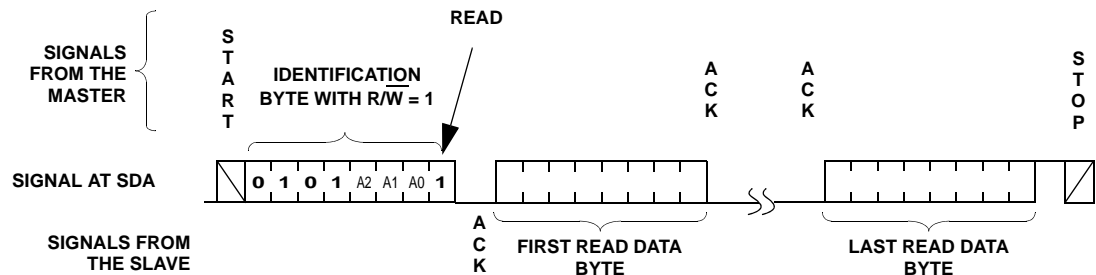
FIGURE 17. ADDRESS READ SEQUENCE
