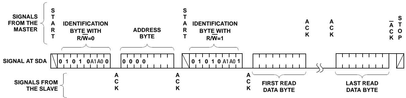
FIGURE 19. READ SEQUENCE
