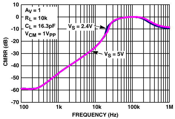
FIGURE 8. CMRR vs FREQUENCY
