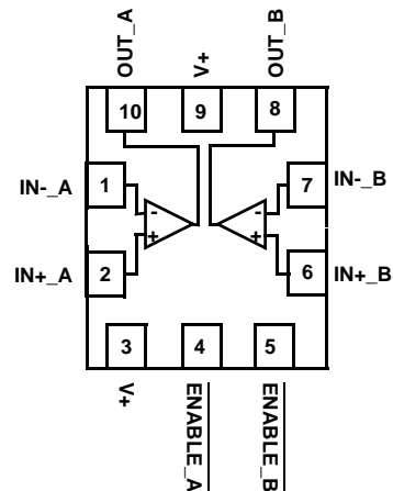
ISL28290 (10 Ld \mu TQFN) TOP VIEW
