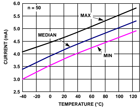
FIGURE 16. SUPPLY CURRENT vs TEMPERATURE V_S = \pm 2.5V ENABLED. R_L = \infty
