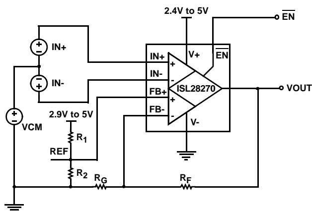
FIGURE 29. GAIN SETTING AND REFERENCE CONNECTION
