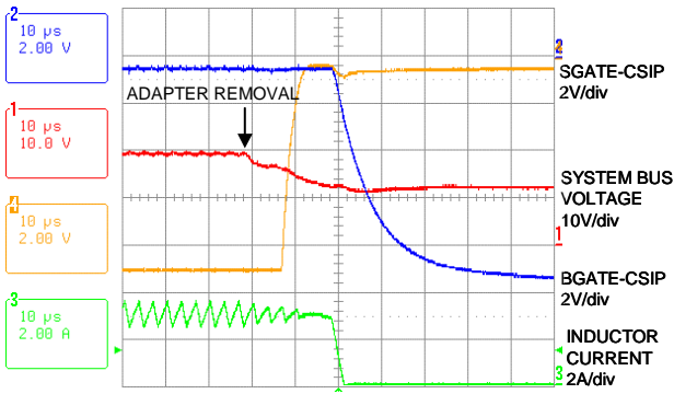
FIGURE 11. SWITCHING WAVEFORMS AT DIODE EMULATION
