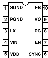
ISL8010 (10 LD MSOP) TOP VIEW
