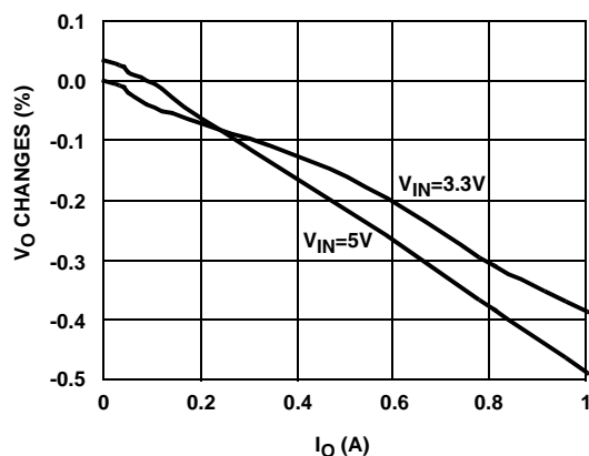
FIGURE 6. LOAD REGULATIONS (PWM MODE)
