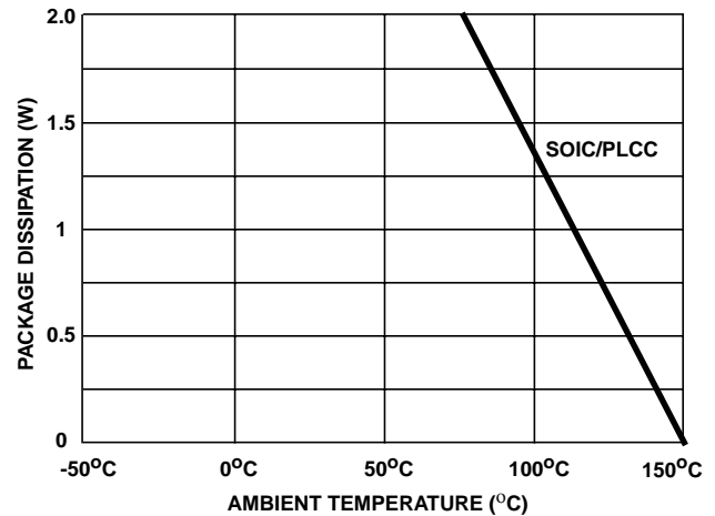
FIGURE 7. MAXIMUM POWER DISSIPATION RATING vs TEMPERATURE FOR THE CA3272AQ, CA3292AQ PLCC PACKAGE AND THE CA3272AM, CA3292AM SOIC PACKAGE WITH 2 SQ. IN. OF 1 OZ. COPPER PC BOARD AREA FOR HEAT SINKING
