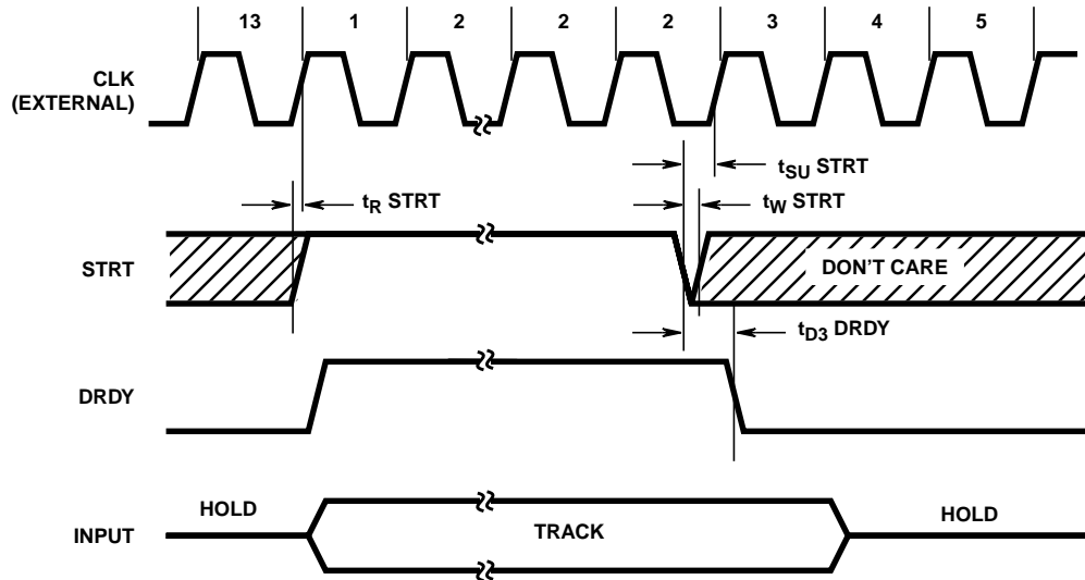
FIGURE 4. STRT PULSED LOW, DRST TIED HIGH, EXTERNAL CLOCK
