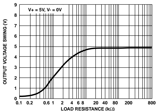
FIGURE 25. OUTPUT SWING vs LOAD RESISTANCE
