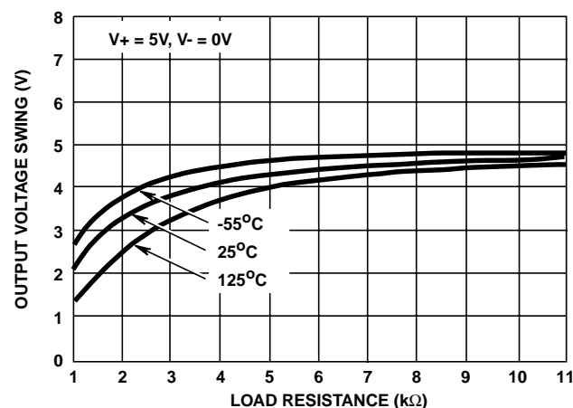
FIGURE 24. OUTPUT VOLTAGE SWING vs LOAD RESISTANCE
