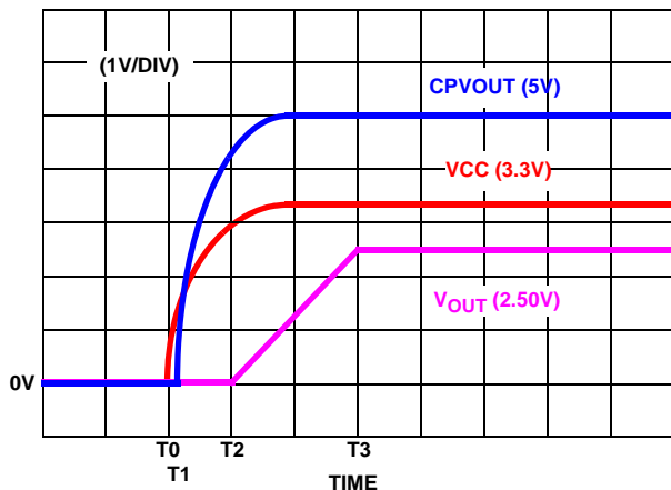
FIGURE 1. SOFT-START INTERVAL
