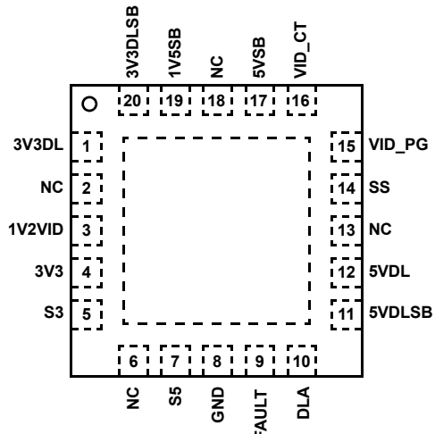
ISL6504/A (6 x 6 QFN) TOP VIEW
