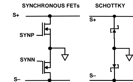
FIGURE 17A. CURRENT DOUBLER RECTIFIERS
