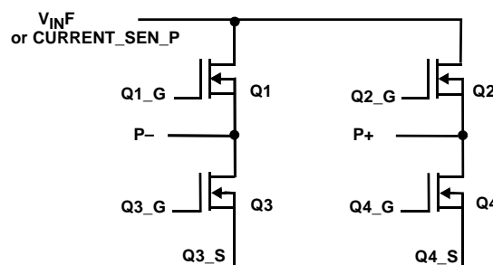
FIGURE 15A. FULL BRIDGE
