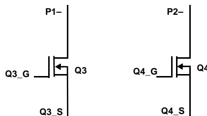
FIGURE 15B. PUSH-PULL
