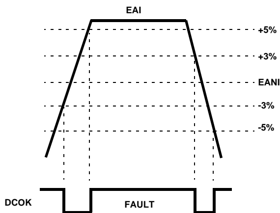
FIGURE 11. UNDERVOLTAGE-OVERVOLTAGE WINDOW
