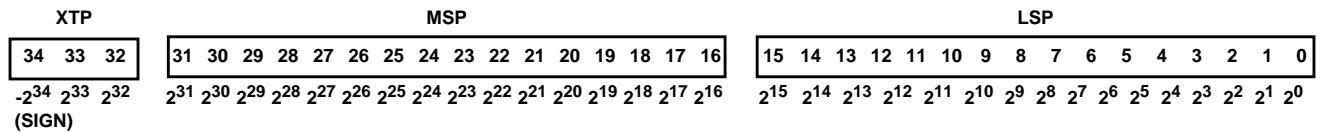
FIGURE 6. TWO'S COMPLEMENT INTEGER OUTPUT
