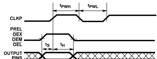
FIGURE 12. PRELOAD TIMING DIAGRAM
