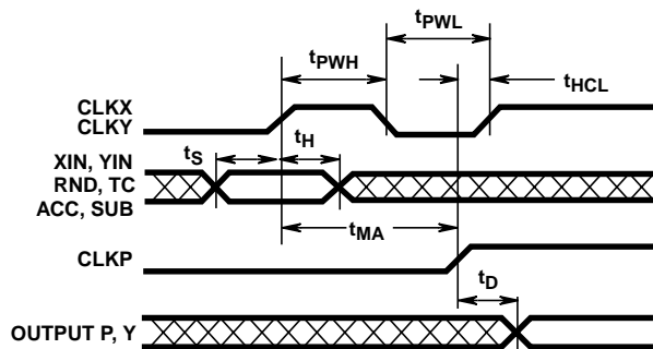
FIGURE 11. HMA510 TIMING DIAGRAM
