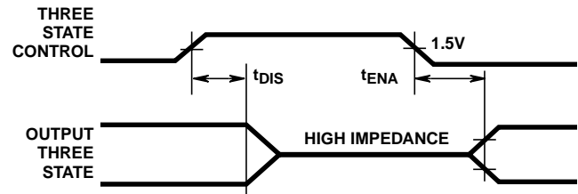
FIGURE 10. THREE-STATE CONTROL
