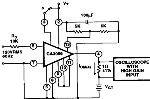
FIGURE 5(a). PEAK OUTPUT CURRENT (PULSED) WITH EXTERNAL POWER SUPPLY TEST CIRCUIT FOR CA3059
