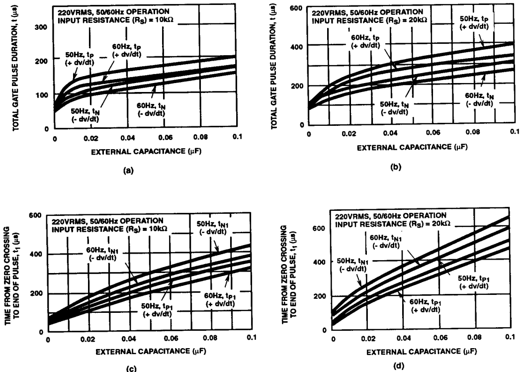
FIGURE 10. RELATIVE PULSE WIDTH AND LOCATION OF ZERO CROSSING FOR 220 VOLT OPERATION FOR CA3059 AND CA3079
