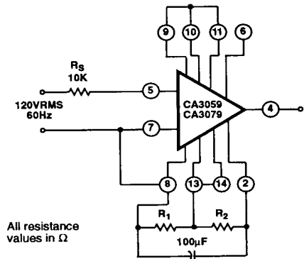
FIGURE 6(a). INPUT INHIBIT VOLTAGE RATIO TEST CIRCUIT FOR CA3059 AND CA3079
