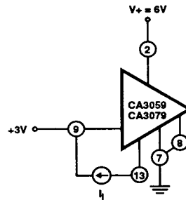
FIGURE 9. INPUT BIAS CURRENT TEST CIRCUIT FOR CA3059 AND CA3079
