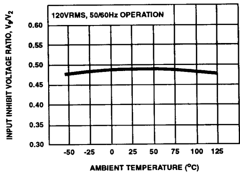
FIGURE 6(b). INPUT INHIBIT VOLTAGE RATIO vs. AMBIENT TEMPERATURE FOR CA3059 AND CA3079
