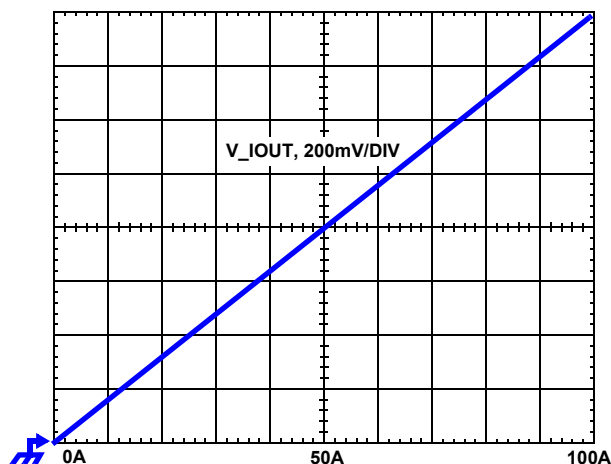
FIGURE 17. VOLTAGE AT IOUT PIN WITH A NTC NETWORK PLACED BETWEEN IOUT TO GROUND WHEN LOAD CURRENT CHANGES
