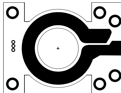
FIGURE 4B. INT. LAYER 1: 1 TURN SECONDARY WINDING
