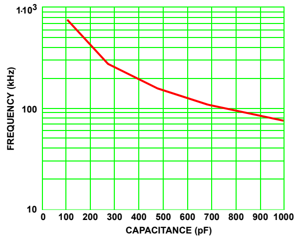
FIGURE 3. CAPACITANCE vs FREQUENCY (RTD = 51.1kΩ)
