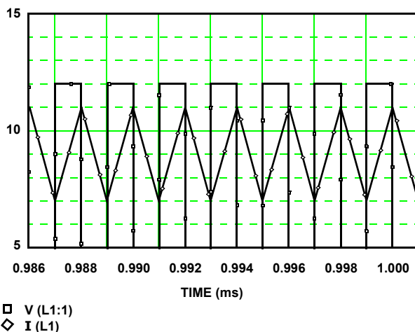
FIGURE 6. SECONDARY WINDING VOLTAGE AND INDUCTOR CURRENT DURING CURRENT LIMIT OPERATION
