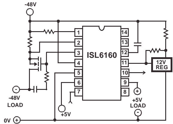
FIGURE 3. -48V/+5V APPLICATION CIRCUIT
