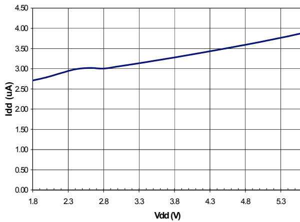
FIGURE 9. I_{DD3} vs V_{DD}
