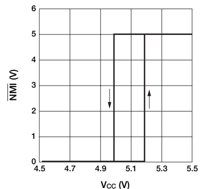
■ \overline{NMI} Judge Voltage Characteristics
