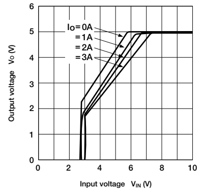
Rise Characteristics
