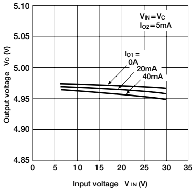
Line Regulation (1)
