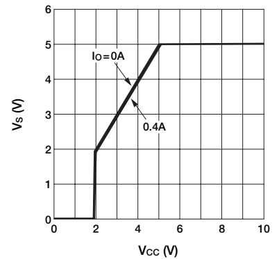
■ V_S Rise Characteristics
