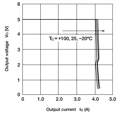
Overcurrent Protection Temperature Characteristics
