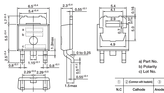
2: (TO-220S)
