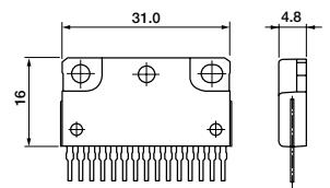
SLA15pin
