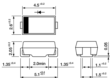
1: (Surface-mount SFP)
