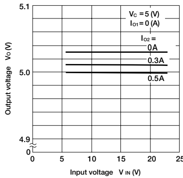
Line Regulation (2)
