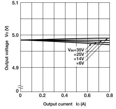
■ Load Regulation
