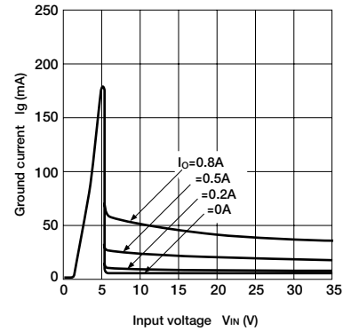
■ Circuit Current
