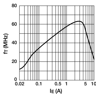
■ f T —I E Characteristics (typ.)
