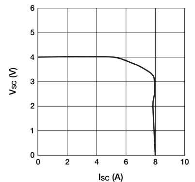
■ V_{SC} Overcurrent Protection Characteristics
