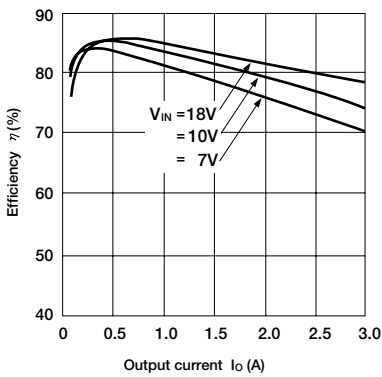
Efficiency Curve
