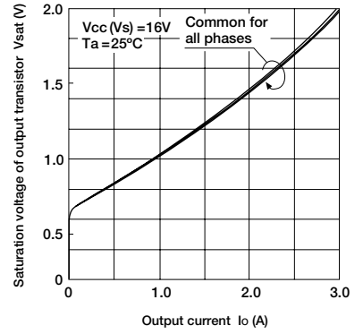
■ Saturation Voltage of Output Transistor Characteristics
