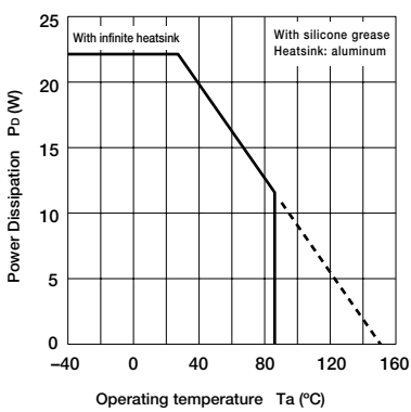
Ta—Pd Characteristics
