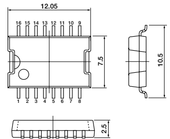
SPF16pin
