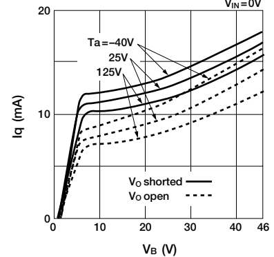
■ Quiescent Circuit Current (dual circuit)
