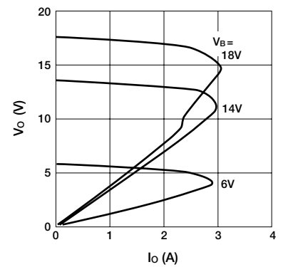
■ Overcurrent Protection Characteristics ( T_a = 25^\circ\text{C} )
