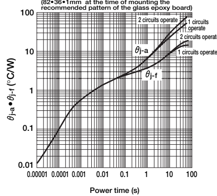
■ Transient thermal resistance characteristics (82×36×1mm at the time of mounting the recommended pattern of the glass epoxy board)
