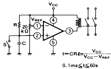
(2) CR Timer
