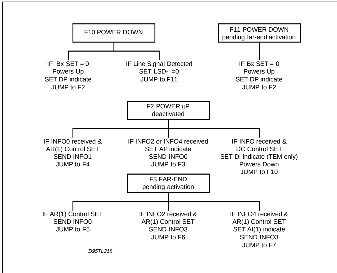
Figure 6: Activation Procedure in GCI mode, TE Selected
