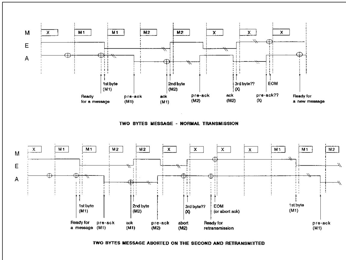
Figure 4: Monitor messaging
