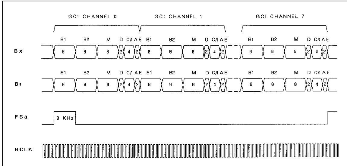
Figure 3: GCI Interface Structure
