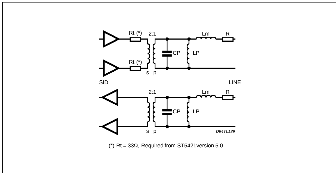
Figure 9: Transmit & Receive Transformer Model
