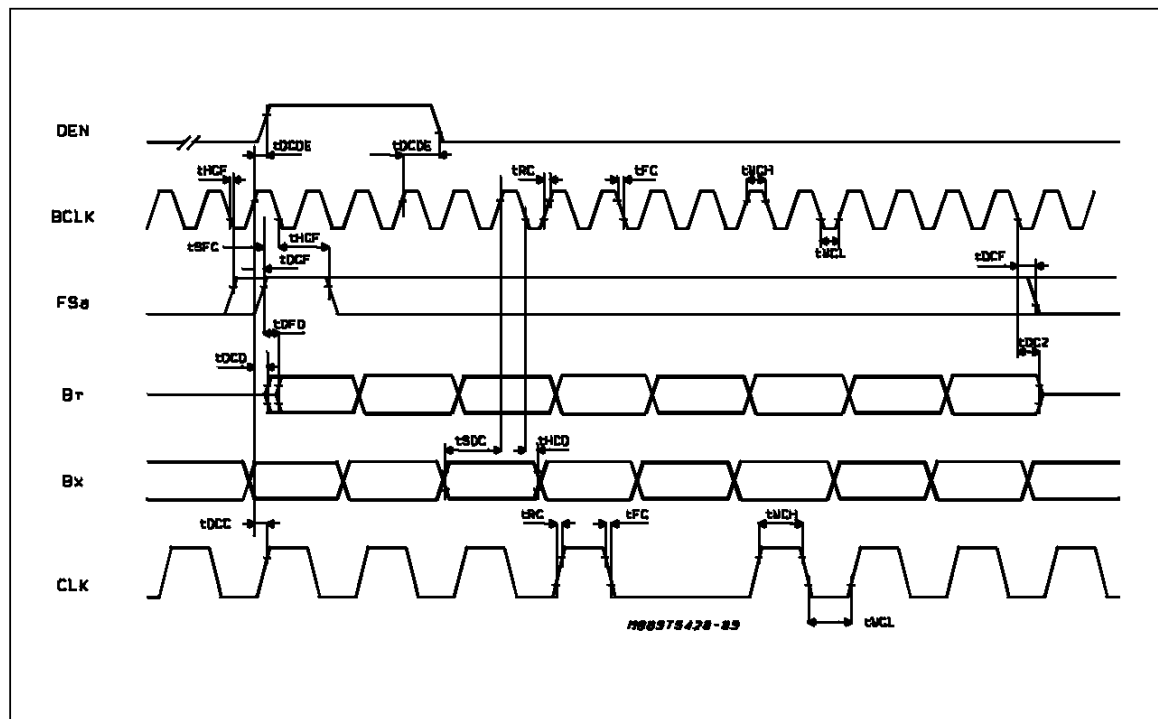
Figure 10: GCI Mode
