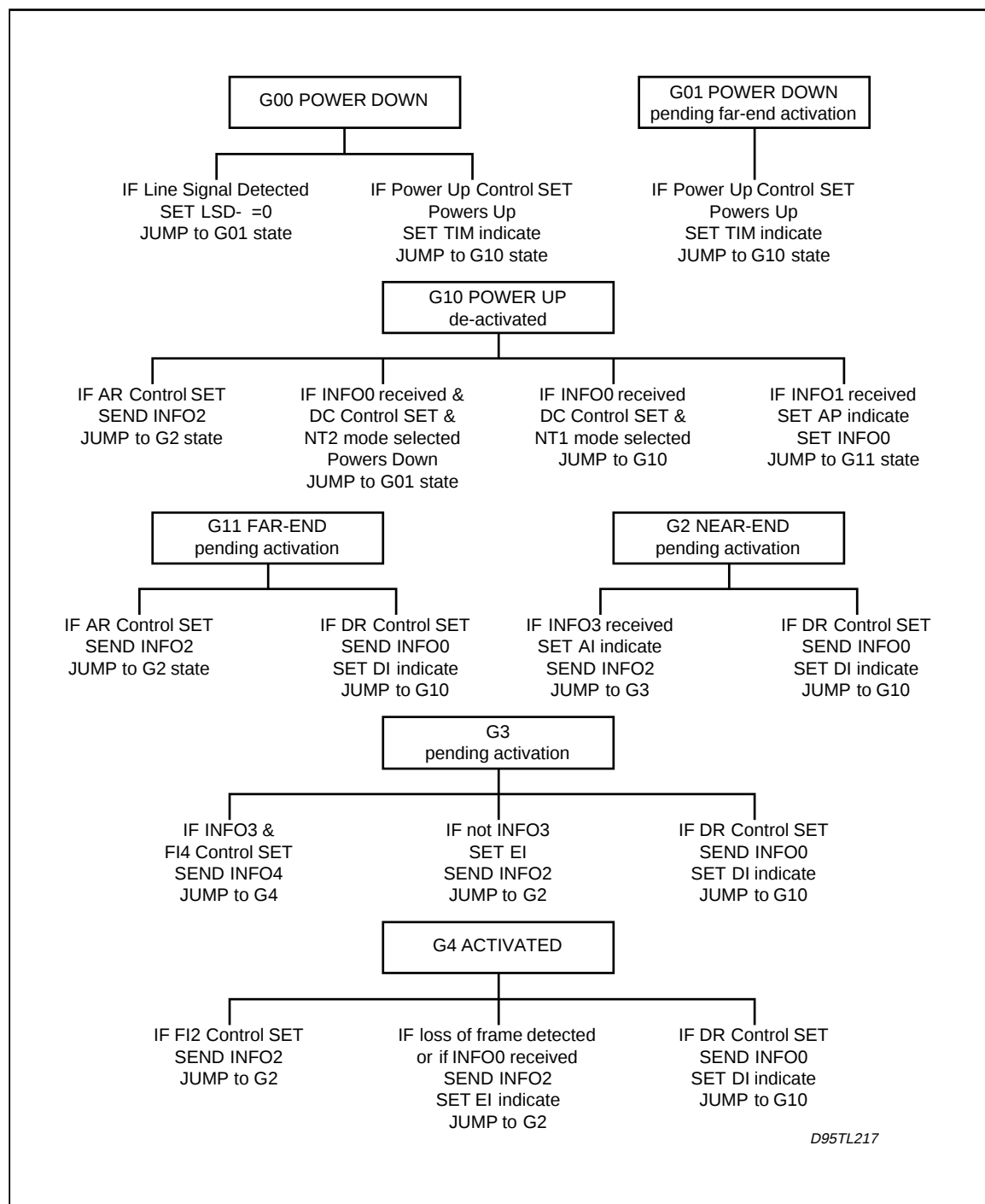
Figure 5: Activation Procedure in GCI mode, NT Selected.
