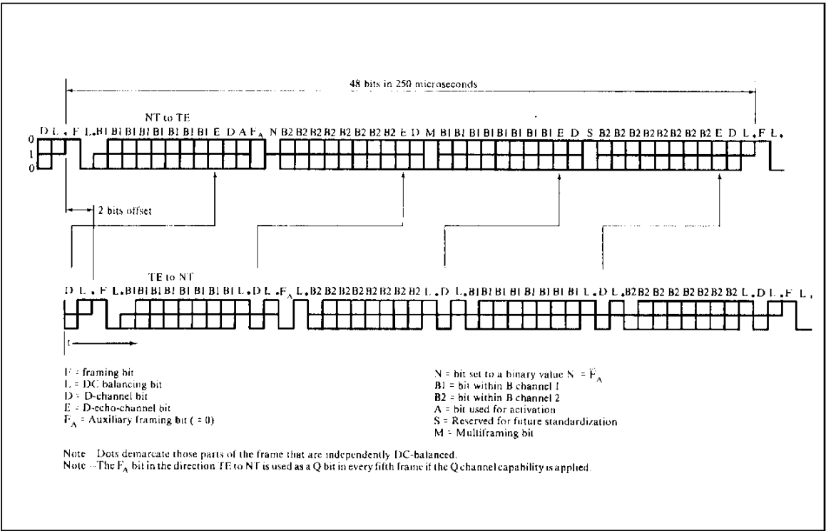
Figure 2: Frame Format
