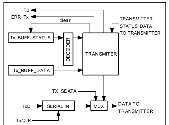
Figure H2 : Tx Buffer Schematics
