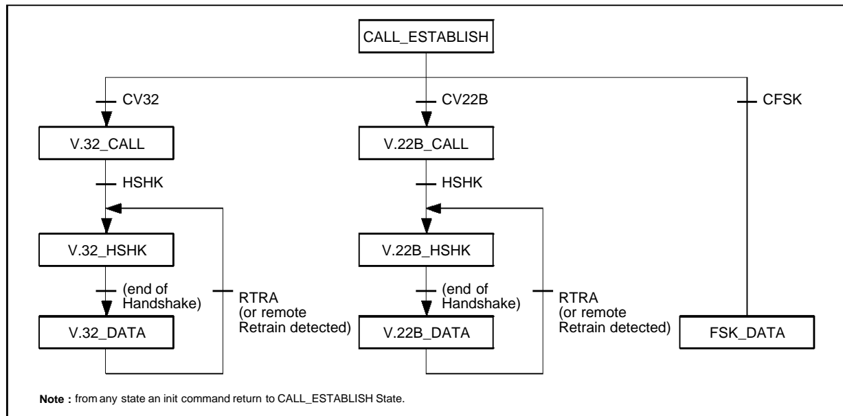
Figure 9 : State Diagram
