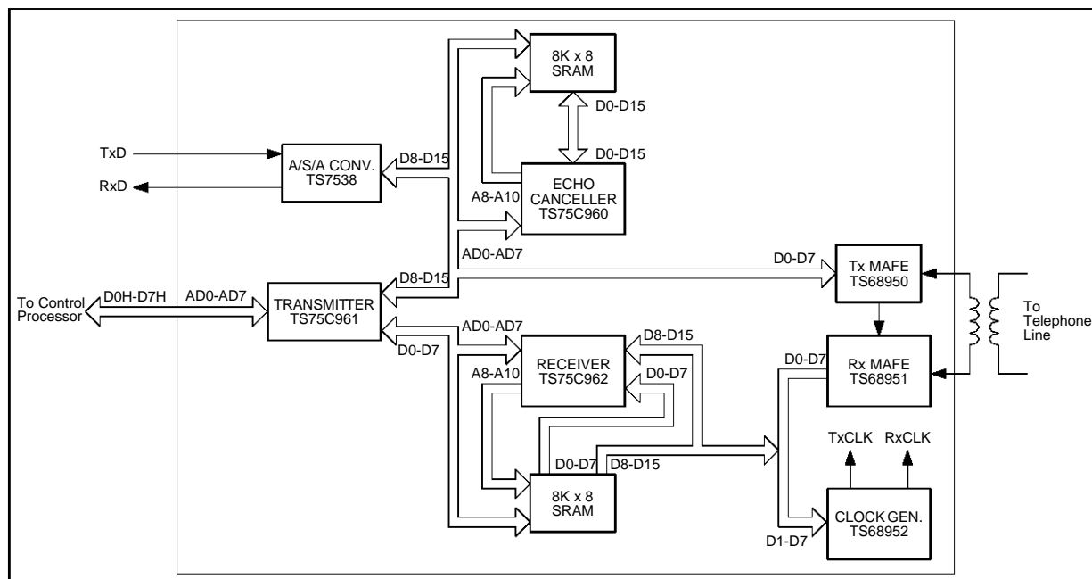
Figure 5 : Hardware Architecture
