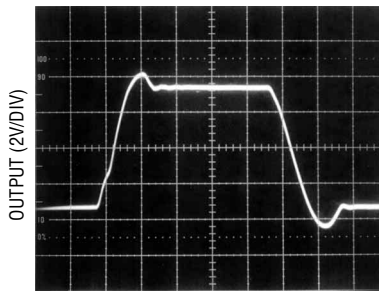
Large-Signal Transient Response ( I_S = 3mA per Amplifier)
