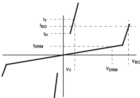
FIGURE 1. V-I CHARACTERISTICS
