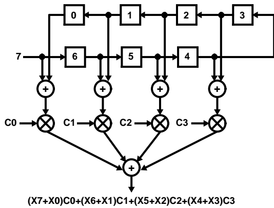
A. DATA FLOW AS DATA SAMPLE 7 IS CLOCKED INTO THE FEED FORWARD STAGE
