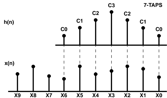
FIGURE 9. DATA/COEFFICIENT ALIGNMENT FOR 7-TAP SYMMETRIC FILTER
