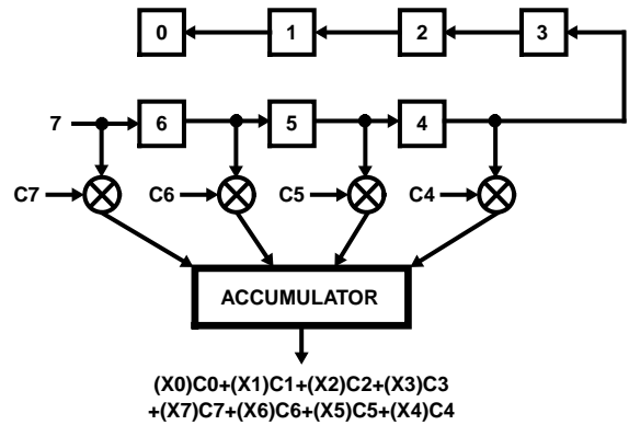
B. SHIFTING OF DATA SAMPLE 7 INTO FIR CELL ENABLED, FORWARD SHIFTING REGISTERS FEEDING MULTIPLIERS
