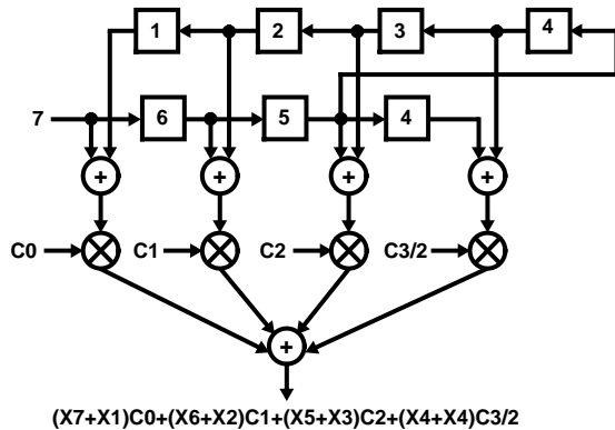
B. DATA FLOW AS DATA SAMPLE 7 IS CLOCKED INTO THE FEED FORWARD STAGE
