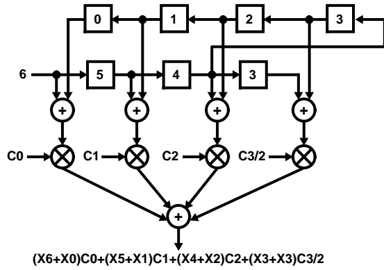
A. DATA FLOW AS DATA SAMPLE 6 IS CLOCKED INTO THE FEED FORWARD STAGE
