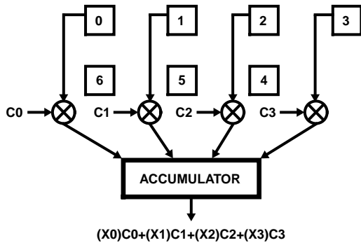
A. DATA SHIFTING DISABLED, BACKWARD SHIFTING DECIMATION REGISTERS FEEDING MULTIPLIERS
