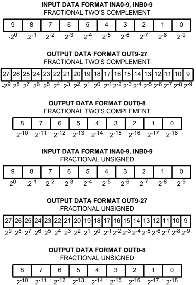
FIGURE 3. INPUT/OUTPUT FORMAT DEFINITIONS
