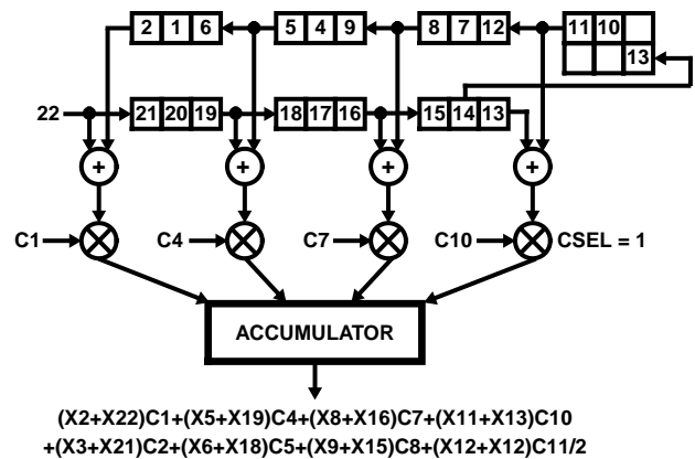
B. COMPUTATIONAL FLOW AS DATA SAMPLE 22 IS CLOCKED INTO THE FEED FORWARD STAGE
