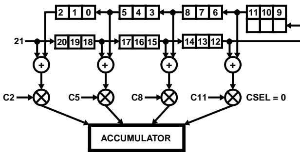
A. COMPUTATIONAL FLOW AS DATA SAMPLE 21 IS CLOCKED INTO THE FEED FORWARD STAGE
