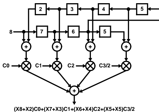
C. DATA FLOW AS DATA SAMPLE 8 IS CLOCKED INTO THE FEED FORWARD STAGE
