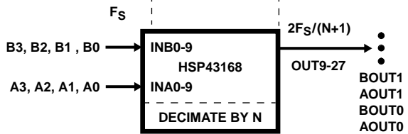
FIGURE 23. MULTIPLEXED DECIMATION BLOCK DIAGRAM
