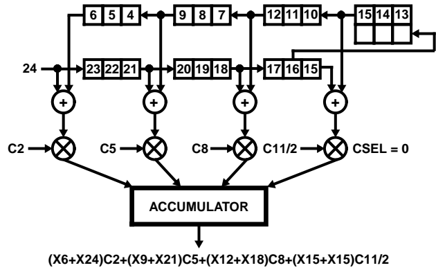
D. COMPUTATIONAL FLOW AS DATA SAMPLE 24 IS CLOCKED INTO THE FEED FORWARD STAGE TXFR TAKES AFFECT ON THIS CLOCK CYCLE
