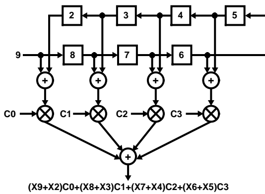
C. DATA FLOW AS DATA SAMPLE 9 IS CLOCKED INTO THE FEED FORWARD STAGE
