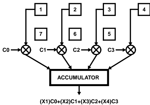
C. DATA SHIFTING DISABLED, BACKWARD SHIFTING DECIMATION REGISTERS FEEDING MULTIPLIERS
