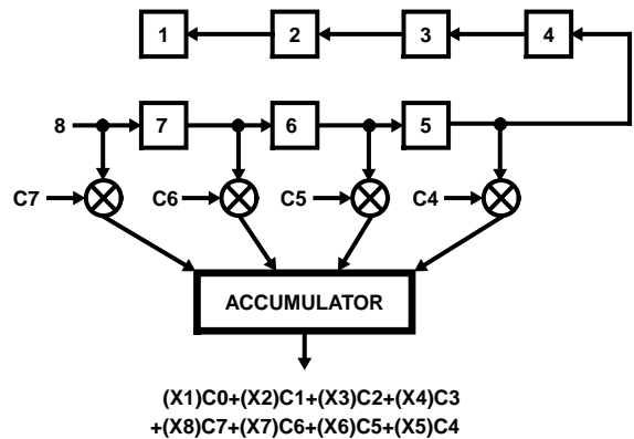
D. SHIFTING OF DATA SAMPLE 8 INTO FIR CELL ENABLED, FORWARD SHIFTING REGISTERS FEEDING MULTIPLIERS
