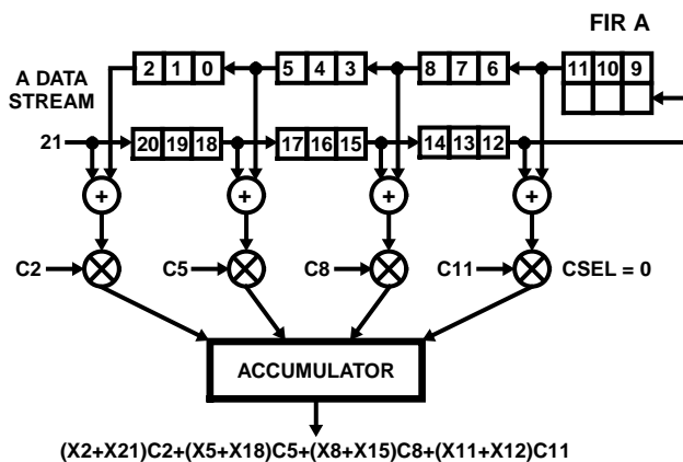
A. COMPUTATIONAL FLOW AS DATA SAMPLE 21 IS CLOCKED INTO THE FEED FORWARD STAGE
