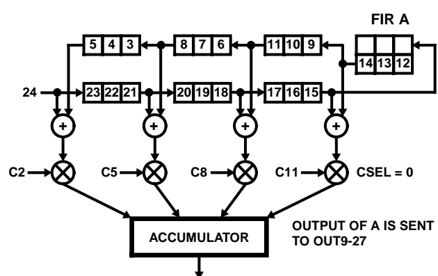
D. COMPUTATIONAL FLOW AS DATA SAMPLE 24 IS CLOCKED INTO THE FEED FORWARD STAGE
