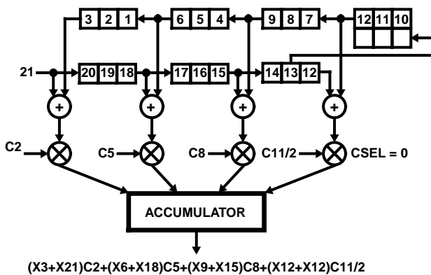
A. COMPUTATIONAL FLOW AS DATA SAMPLE 21 IS CLOCKED INTO THE FEED FORWARD STAGE TXFR TAKES EFFECT ON THIS CLOCK CYCLE
