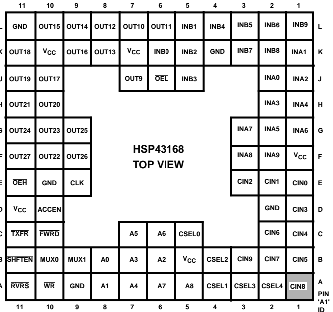
84 LEAD CPGA TOP VIEW
