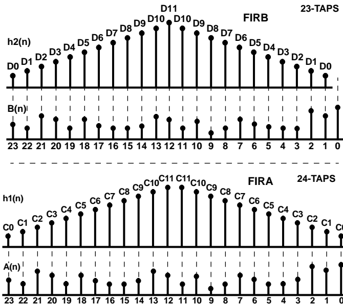
FIGURE 24. DATA/COEFFICIENT ALIGNMENT FOR MULTIPLEXED DECIMATION EXAMPLE
