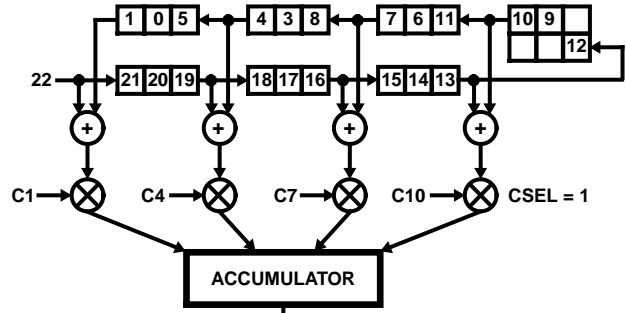
B. COMPUTATIONAL FLOW AS DATA SAMPLE 22 IS CLOCKED INTO THE FEED FORWARD STAGE
