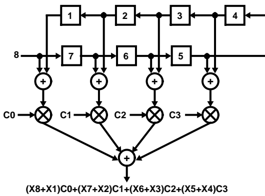
B. DATA FLOW AS DATA SAMPLE 8 IS CLOCKED INTO THE FEED FORWARD STAGE
