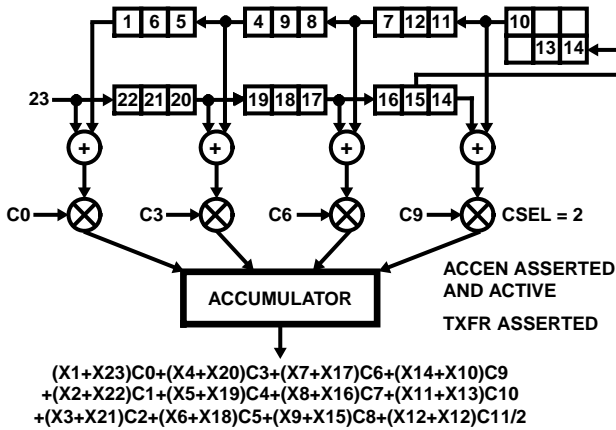
C. COMPUTATIONAL FLOW AS DATA SAMPLE 23 IS CLOCKED INTO THE FEED FORWARD STAGE
