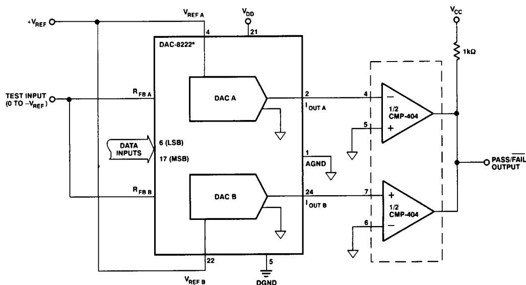
Figure 9. Digitally-Programmable Window Detector (Upper/Lower Limit Detector)
