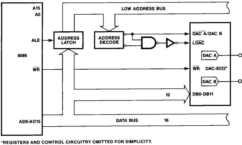
Figure 10. DAC8222 to 8086 Interface
