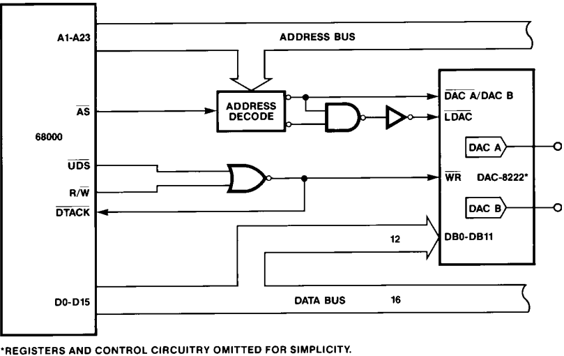
Figure 11. DAC8222 to 68000 Interface
