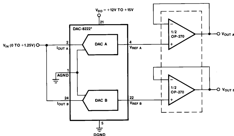
Figure 8. Single Supply Operation (Voltage Switching Mode)
