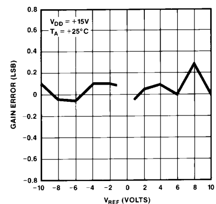
Absolute Gain Error Changes vs. V_{REF}
