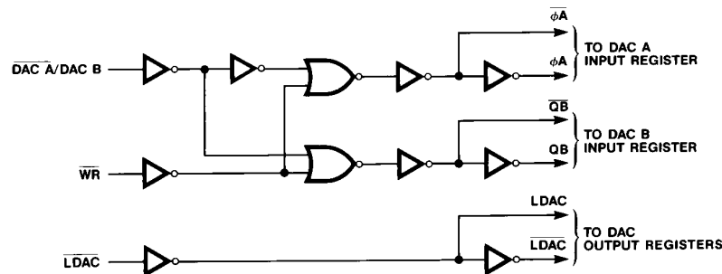
Figure 4. Input Control Logic
