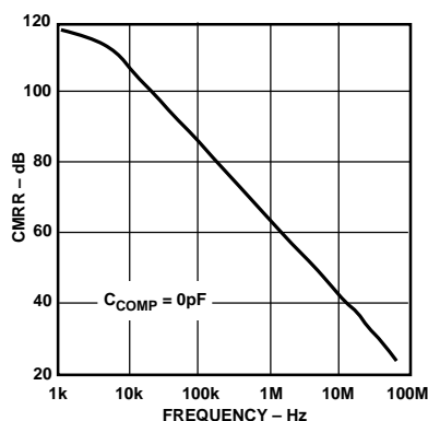
Figure 13. Common-Mode Rejection Ratio vs. Frequency
