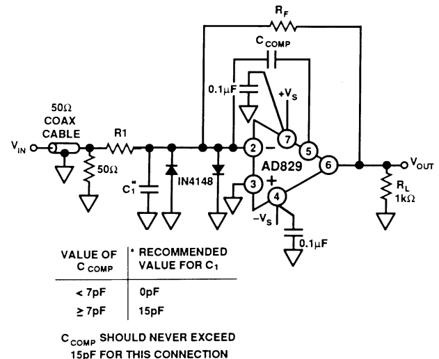
Figure 29. Inverting Amplifier Connection Using Current Feedback Compensation
