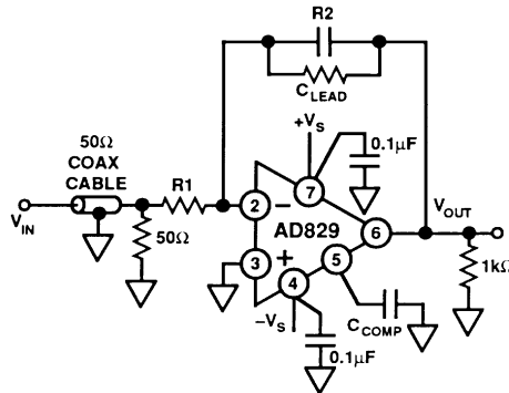
Figure 26. Inverting Amplifier Connection Using External Shunt Compensation
