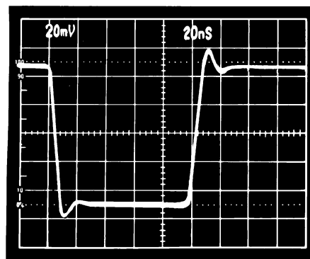
Figure 22c. Gain of 2 Follower Small Signal Pulse Response
