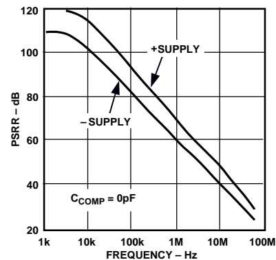
Figure 12. Power Supply Rejection Ratio (PSRR) vs. Frequency
