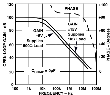
Figure 10. Open-Loop Gain & Phase Margin vs. Frequency
