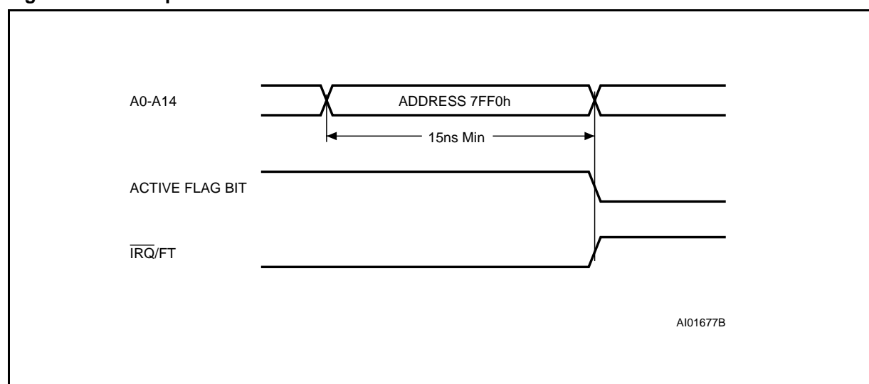
Figure 11. Interrupt Reset Waveforms
