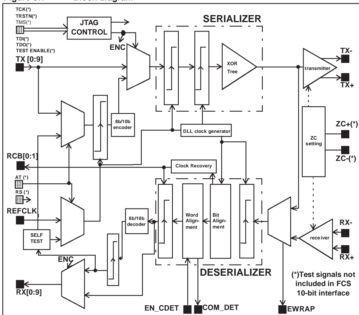
Figure 3.1 Block diagram
