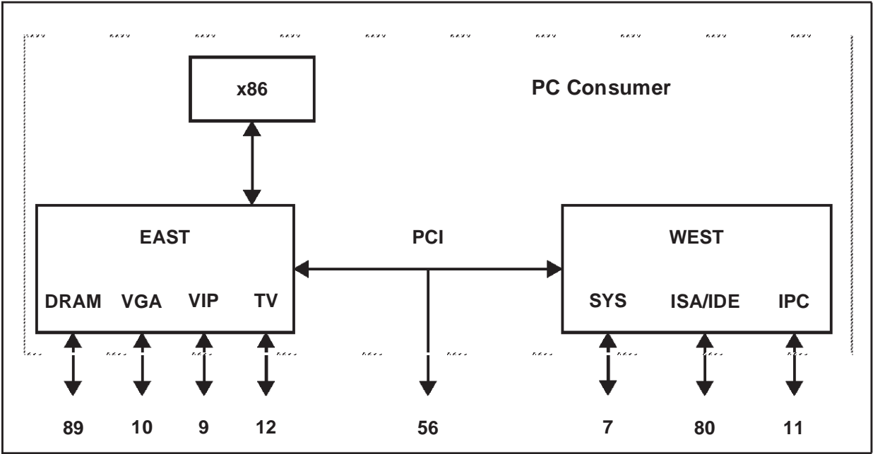
Figure 7. PC Consumer External Interfaces
