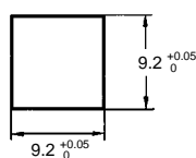
Panel Cutout of B32-12□0
