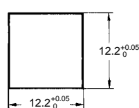
Panel Cutout of B32-12□0
