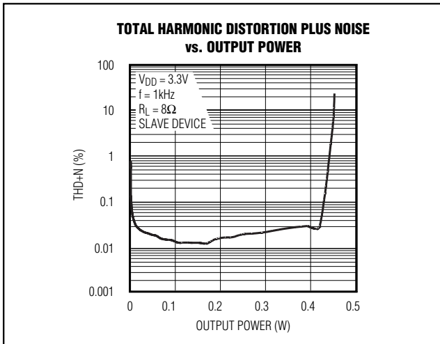
Figure 8. Master-Slave THD+N
