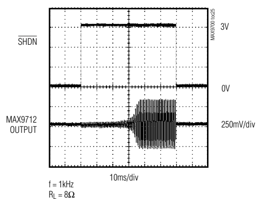
TURN-ON/TURN-OFF RESPONSE
