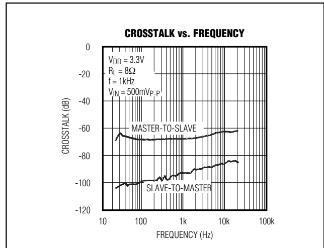
Figure 9. Master-Slave Crosstalk
