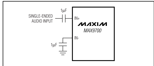
Figure 6. Single-Ended Input
