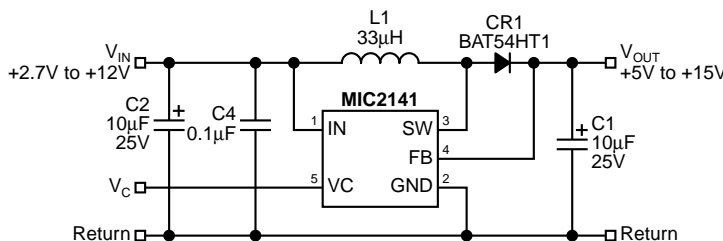
Figure 1. Basic Configuration
