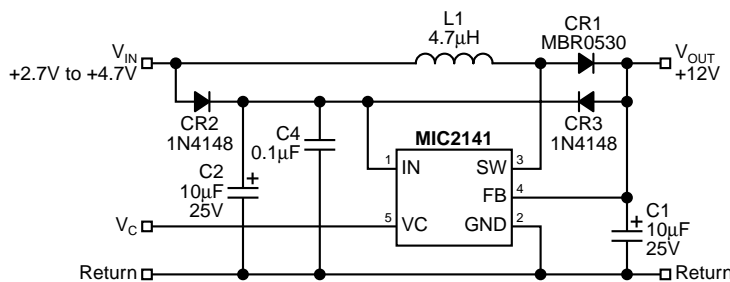
Figure 3. Bootstrap Configuration
