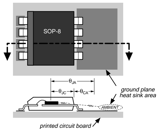
Figure 3. Thermal Resistance
