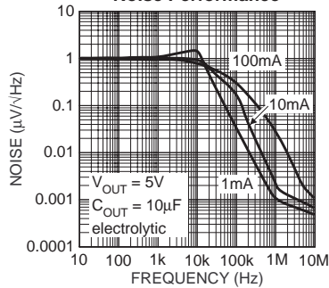
Noise Performance
