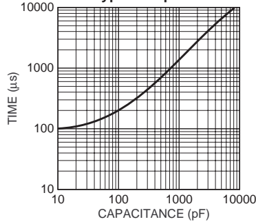
Turn-On Time vs. Bypass Capacitance
