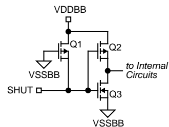
Figure 6b. SHUT
