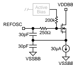
Figure 5. REFOSC Pin
