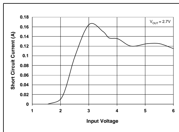
FIGURE 2-5: Short Circuit Current vs. Input Voltage.
