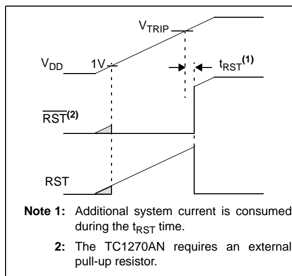
FIGURE 4-7: \overline{RST}/RST pin Operation Power-up.
