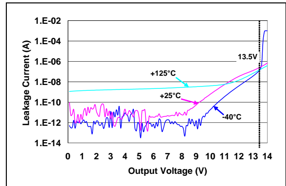
FIGURE 2-41: Open-Drain Leakage Current vs. Voltage Applied to \overline{RST} Pin (TC1270AR, TC1270ANR, TC1271AR - 2.55V minimum).
