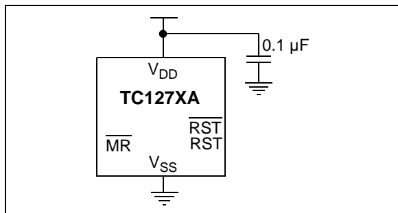
FIGURE 5-1: Typical Application Circuit with Bypass Capacitor.
