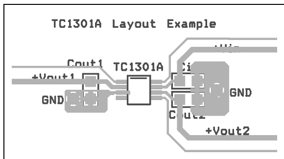
FIGURE 7-2: MSOP8 Wiring Layer.
