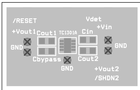
FIGURE 7-3: DFN3X3 Silk-Screen Example.
