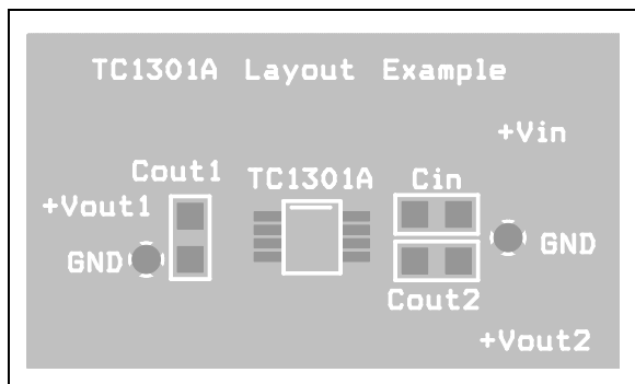
FIGURE 7-1: MSOP8 Silk Screen Layer.
