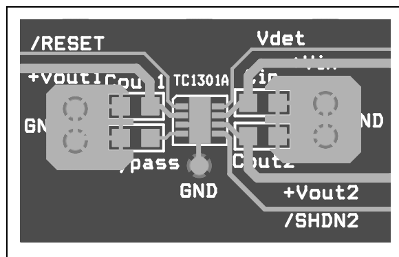
FIGURE 7-4: DFN3X3 Top Metal Layer Example.
