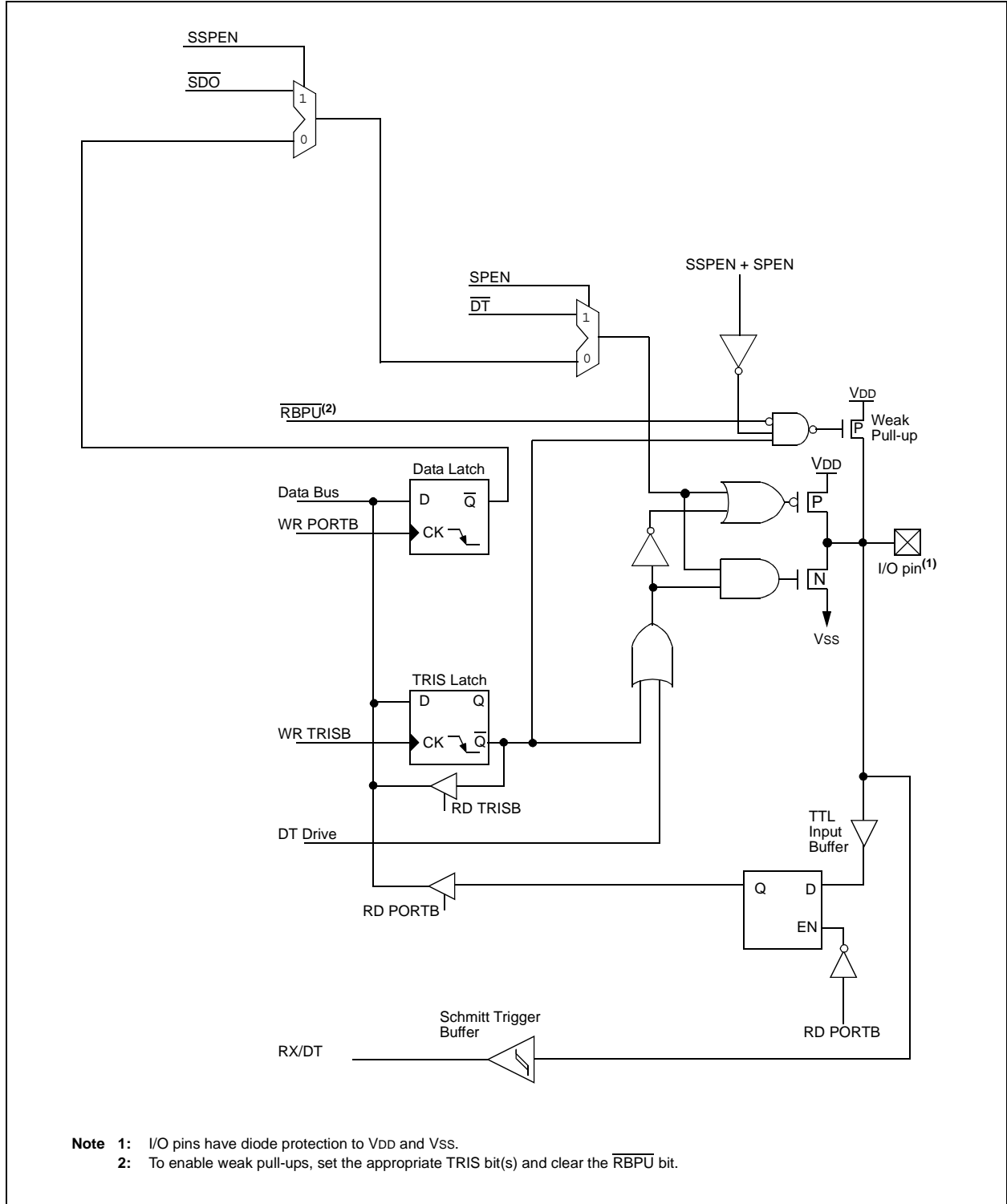
FIGURE 5-10: BLOCK DIAGRAM OF RB2/SDO/RX/DT PIN
