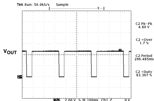
Thermal Shutdown Response of 5.0V LDO
