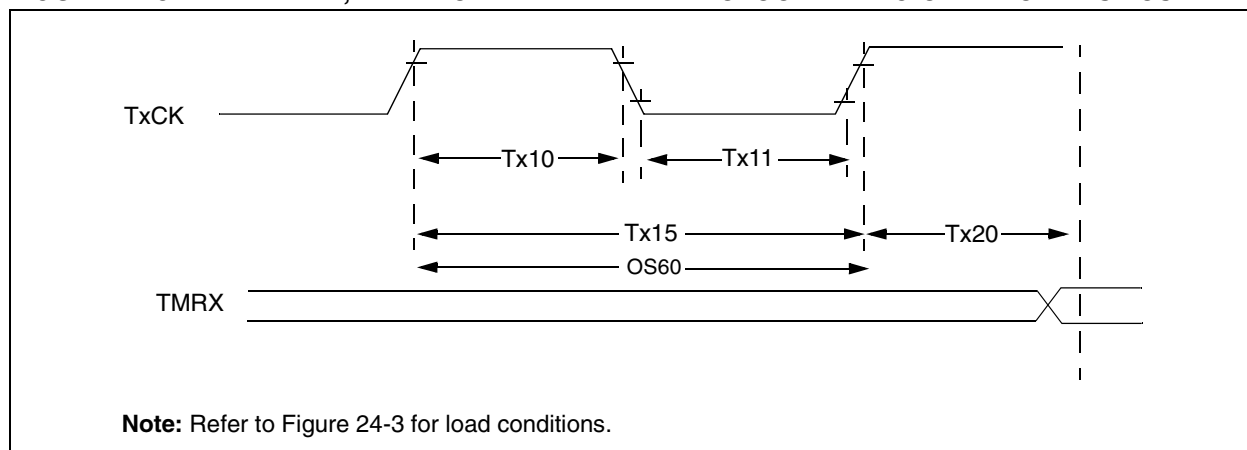
FIGURE 24-8: TYPE A, B AND C TIMER EXTERNAL CLOCK TIMING CHARACTERISTICS
