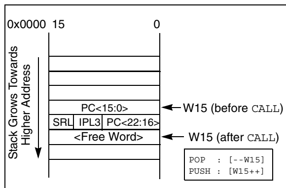
FIGURE 5-2: INTERRUPT STACK FRAME
