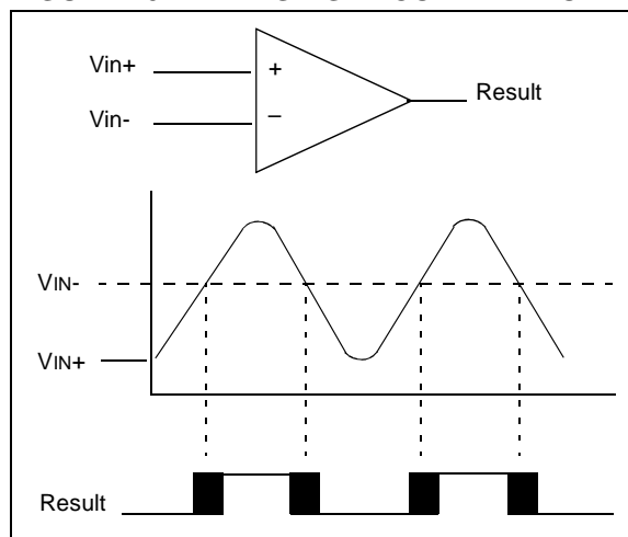
FIGURE 10-2: SINGLE COMPARATOR
