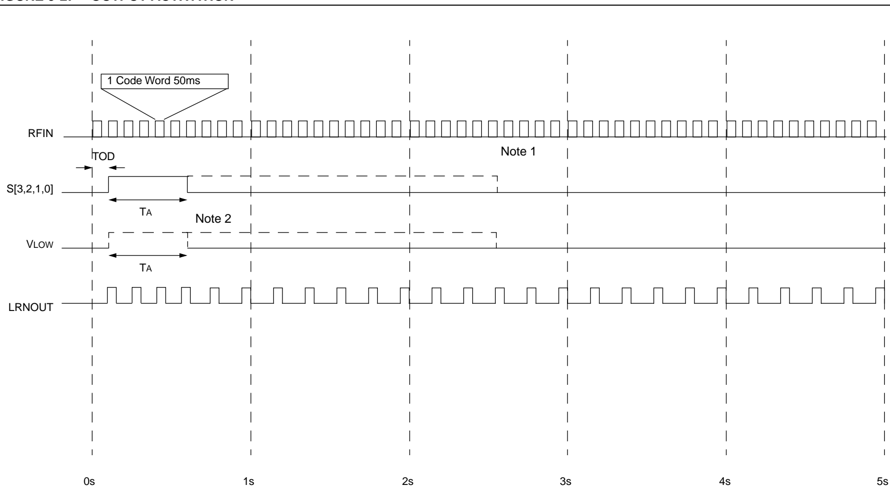
FIGURE 9-2: OUTPUT ACTIVATION
