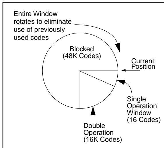
FIGURE 3-3: SYNCHRONIZATION WINDOW
