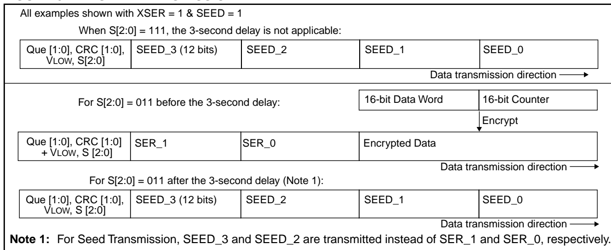
FIGURE 3-1: SEED TRANSMISSION
