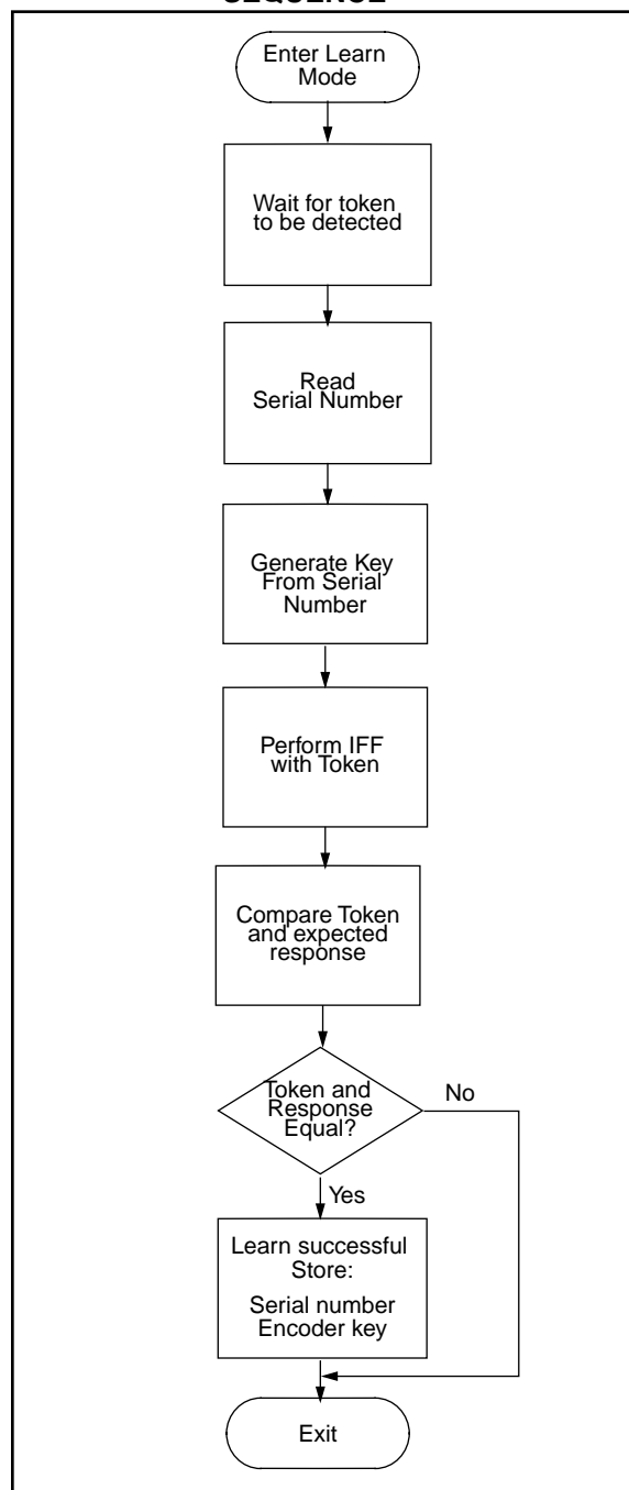
FIGURE 4-3: TYPICAL IFF LEARN SEQUENCE
