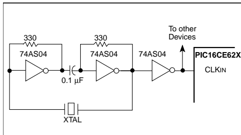
FIGURE 10-5: EXTERNAL SERIES RESONANT CRYSTAL OSCILLATOR CIRCUIT
