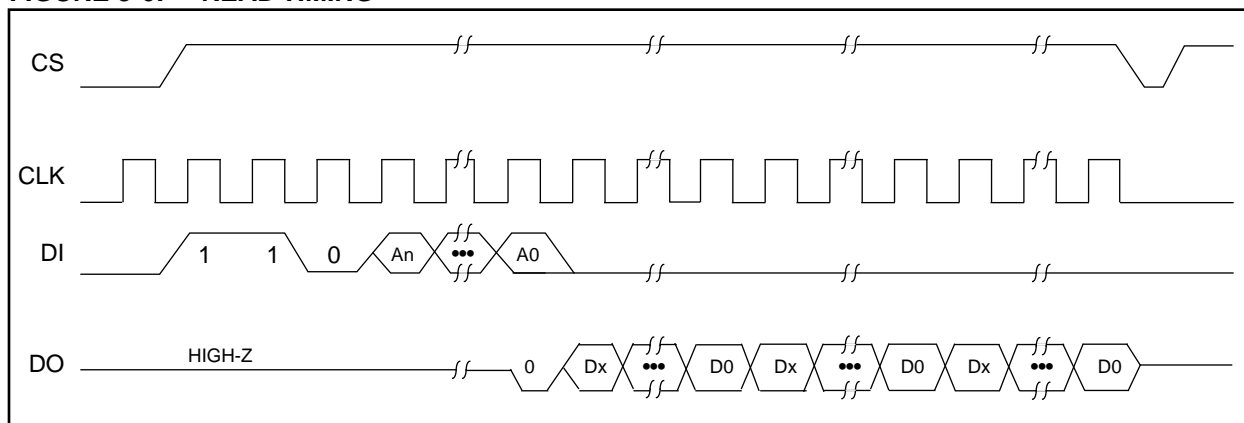
FIGURE 3-6: READ TIMING
