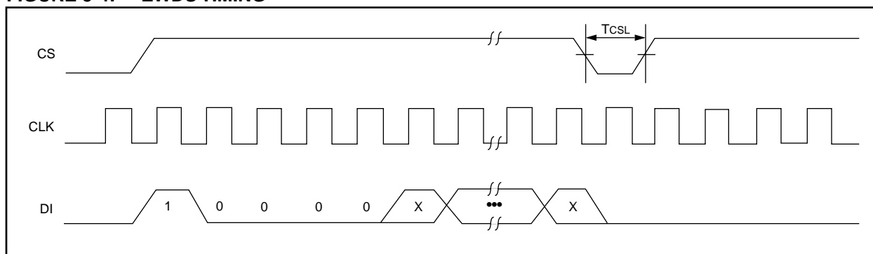
FIGURE 3-4: EWDS TIMING
